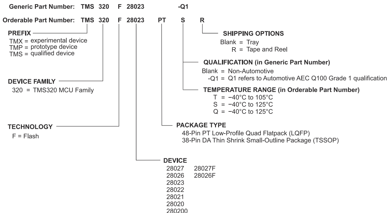
Figure 11-1. Device Nomenclature
