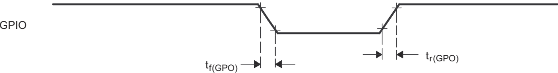
Figure 9-41. General-Purpose Output Timing
