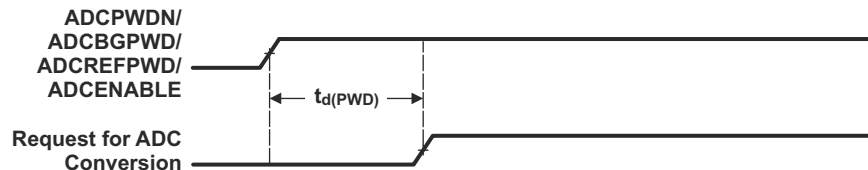
Figure 9-19. ADC Conversion Timing
