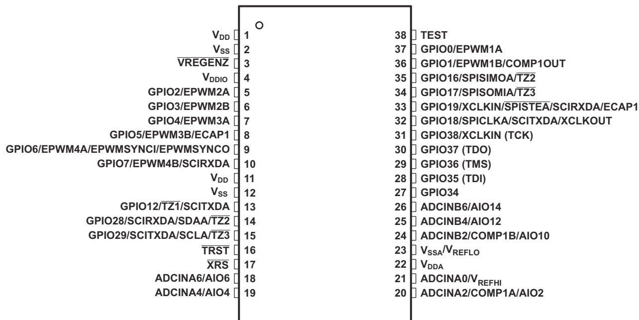
Figure 7-2. 2802x 38-Pin DA TSSOP (Top View)
