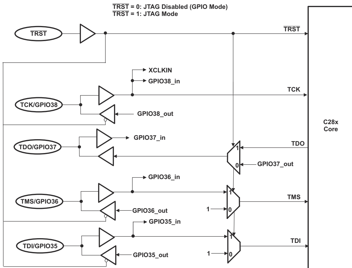
Figure 9-39. JTAG/GPIO Multiplexing
