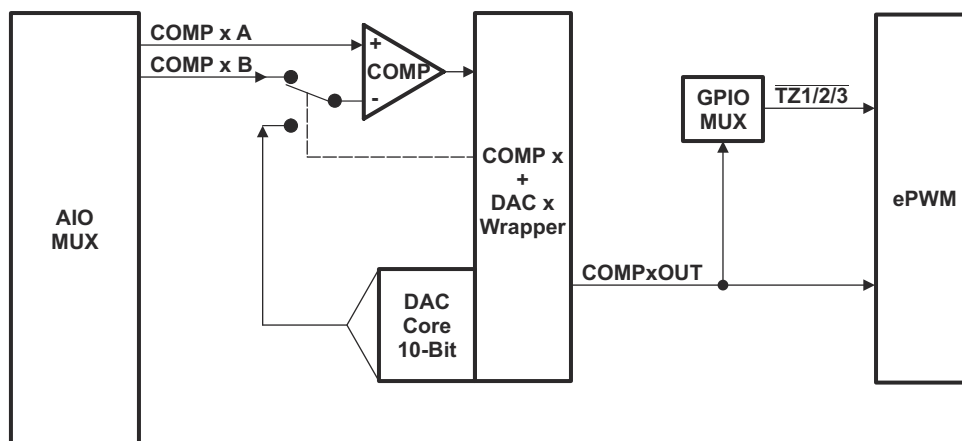
Figure 9-26. Comparator Block Diagram
