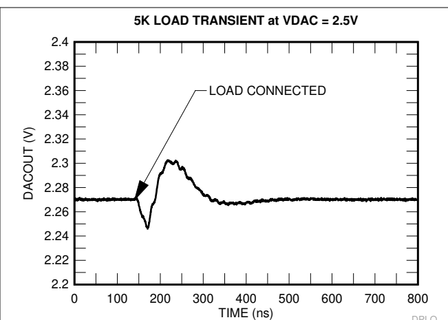
Figure 7-56. 5-k \Omega Load Transient
