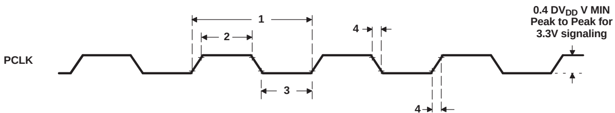
Figure 5-46. PCLK Timing
