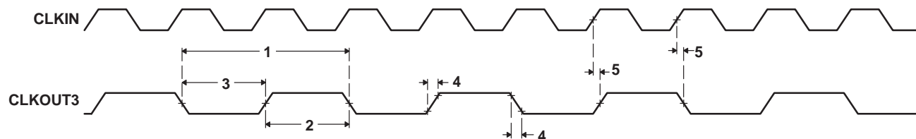
Figure 33. CLKOUT3 Timings
