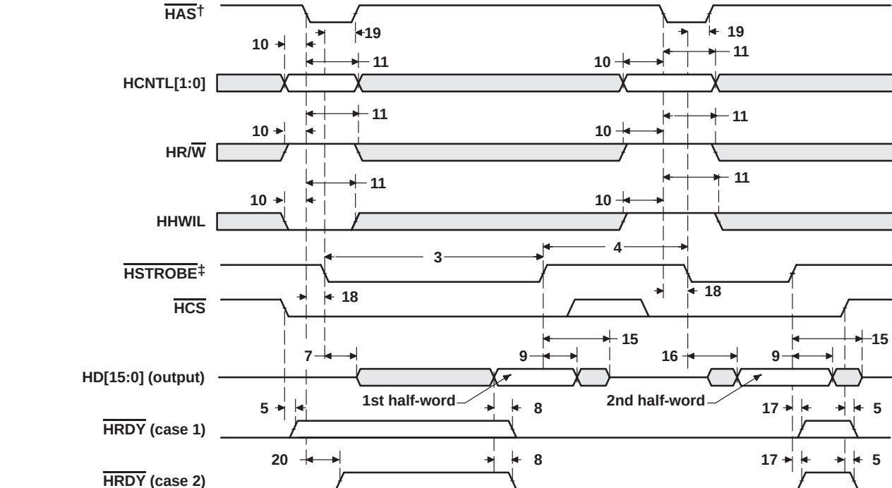
Figure 34. HPI Read Timing ( \overline{\text{HAS}} Used)
