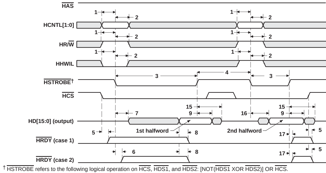
Figure 33. HPI Read Timing ( \overline{\text{HAS}} Not Used, Tied High)
