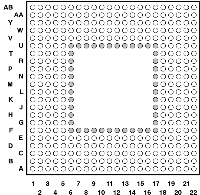
GLS 384-PIN BGA PACKAGE (BOTTOM VIEW) [C6202 only]
