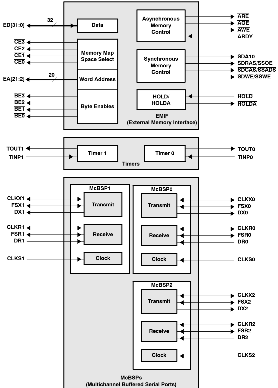
Figure 3. Peripheral Signals
