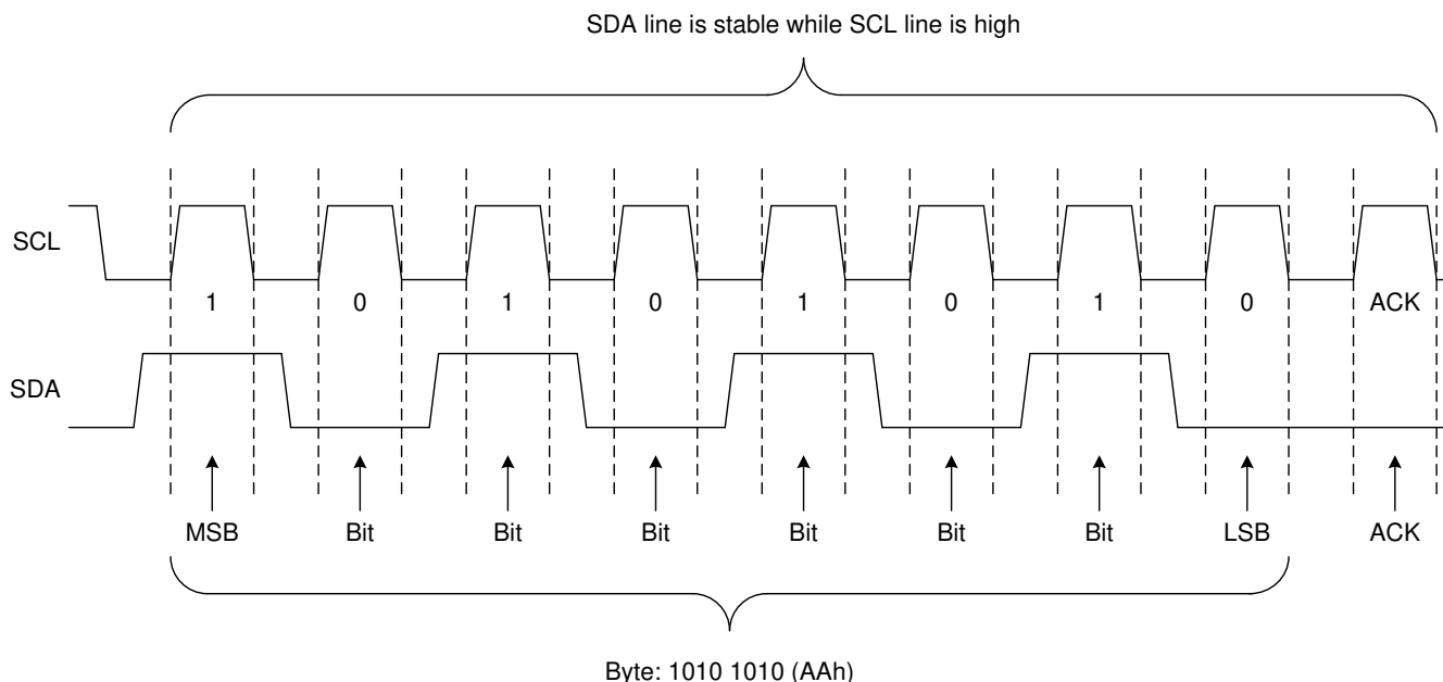
Figure 8-11. Bit Transfer
