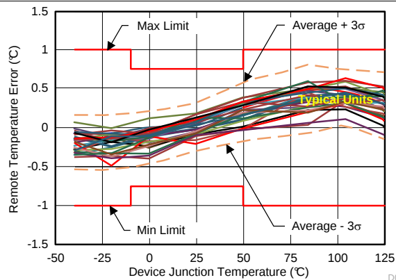
Typical behavior of 30 DSBGA devices over temperature at V_+ = 1.8\text{ V} with the remote diode junction at 150^\circ\text{C} .
