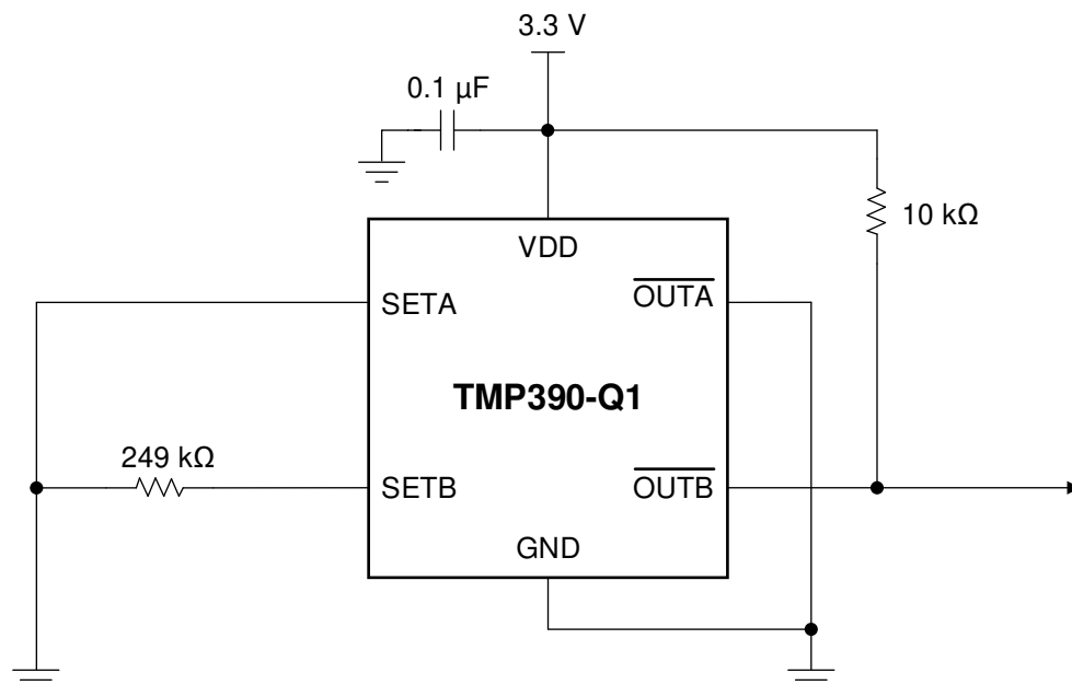
Figure 8-7. TMP390-Q1 One Channel (Cold) Operation Example Circuit With –20°C Trip Point and 10°C Hysteresis
