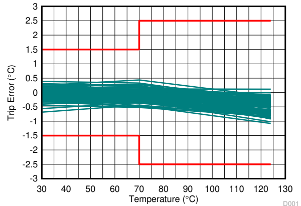
Figure 6-2. Channel A Trip Point Accuracy vs Operating Temperature
