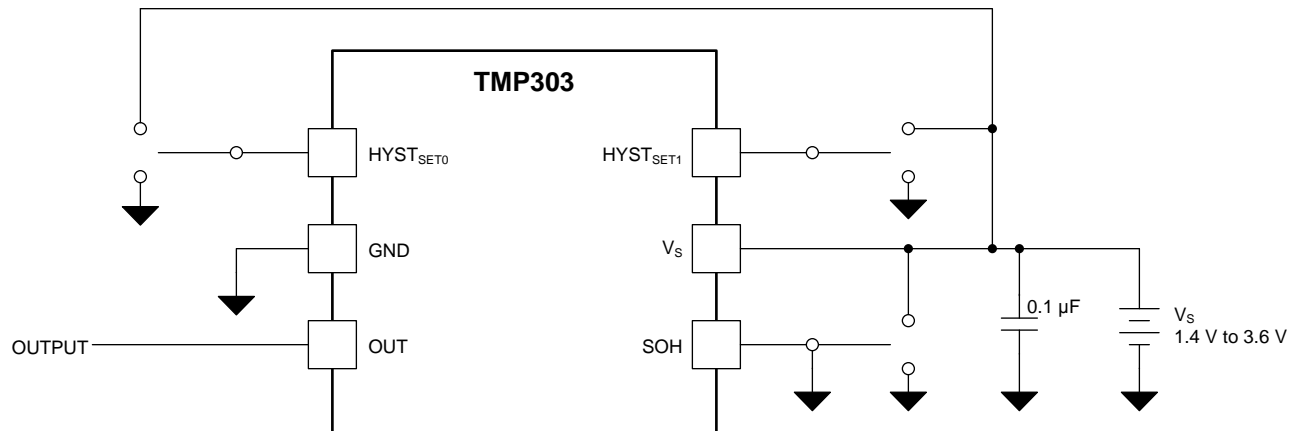
Figure 16. TMP303 With Switches
