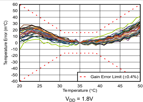
Figure 6-7. Gain Error (Normalized at 35^\circ\text{C} )
