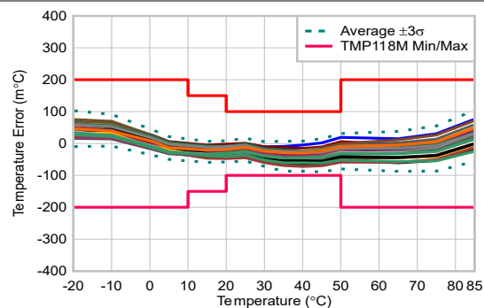
Figure 6-3. TMP118M Temperature Error vs Temperature
