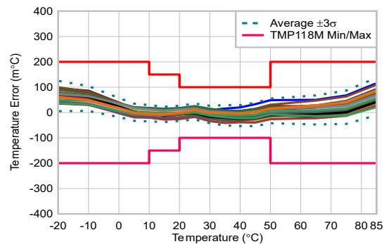
Figure 6-5. TMP118M Temperature Error vs Temperature
