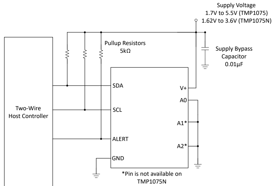
Figure 8-1. Typical Connections
