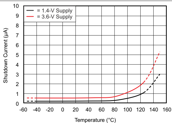
Figure 6-2. Shutdown Current vs Temperature
