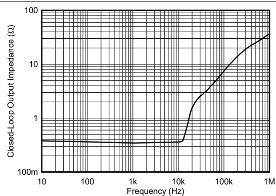
Figure 6-4. Output Impedance vs Frequency
