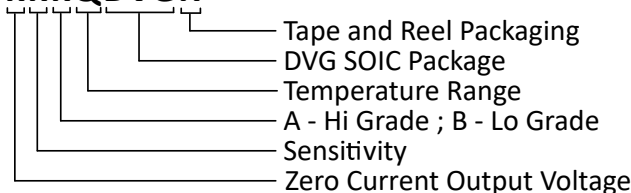
Figure 10-1. Part Number Naming Designators
