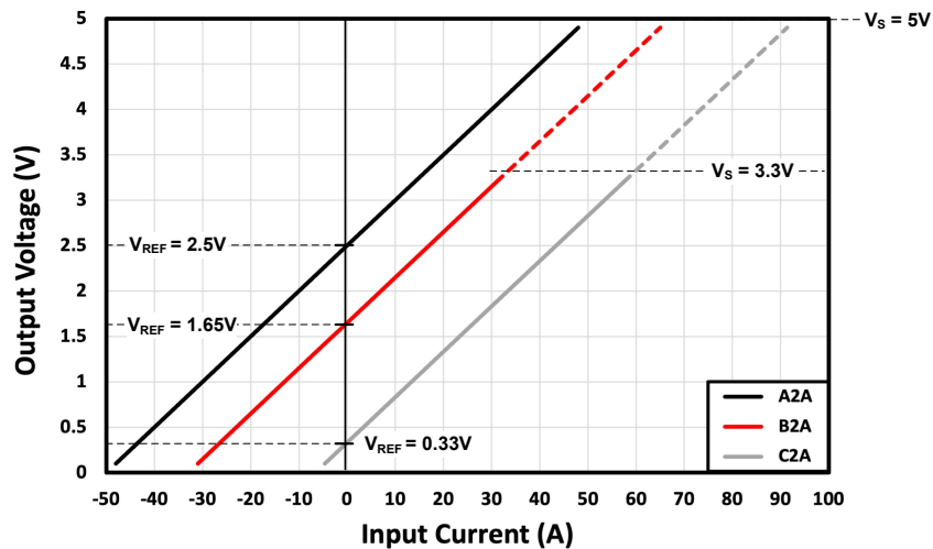
Figure 8-5. Output Voltage Relationship to Input Current for TMCS1123x2A
