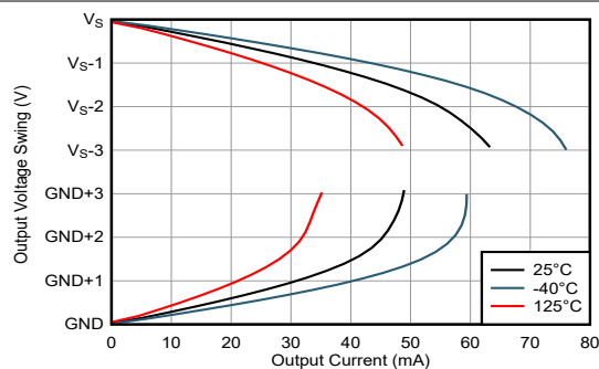
Figure 6-20. Output Swing vs Output Current
