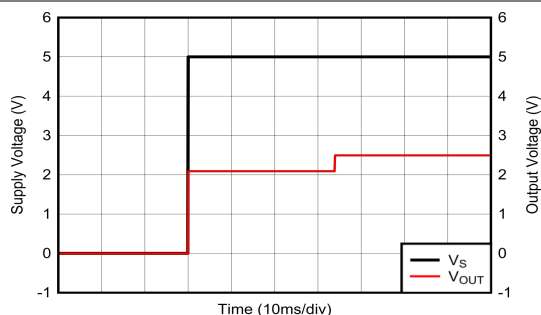
Figure 6-19. Startup Transient Response
