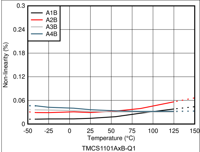
Figure 6-5. Non-Linearity vs Temperature
