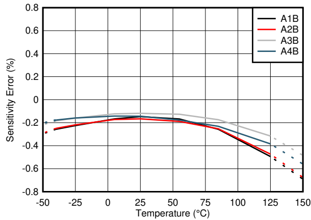
Figure 6-1. TMCS1101AxB-Q1 Sensitivity Error vs Temperature
