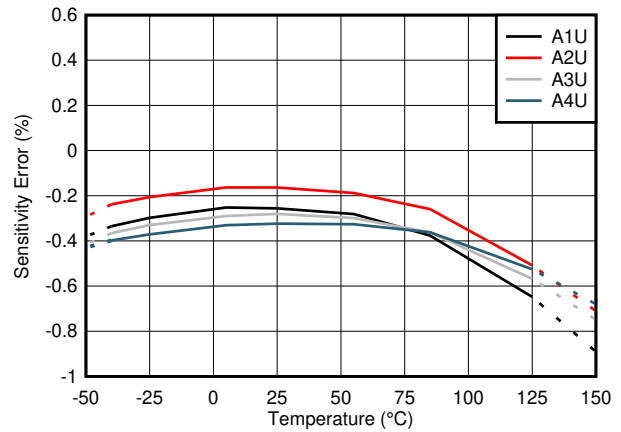
Figure 6-2. TMCS1101AxU-Q1 Sensitivity Error vs Temperature
