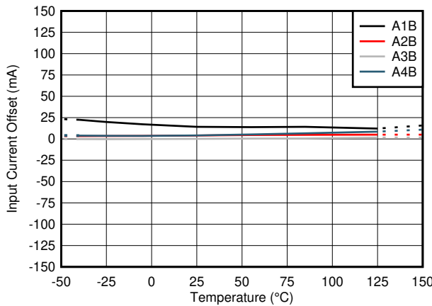
Figure 6-3. TMCS1101AxB-Q1 Input Offset Current vs Temperature
