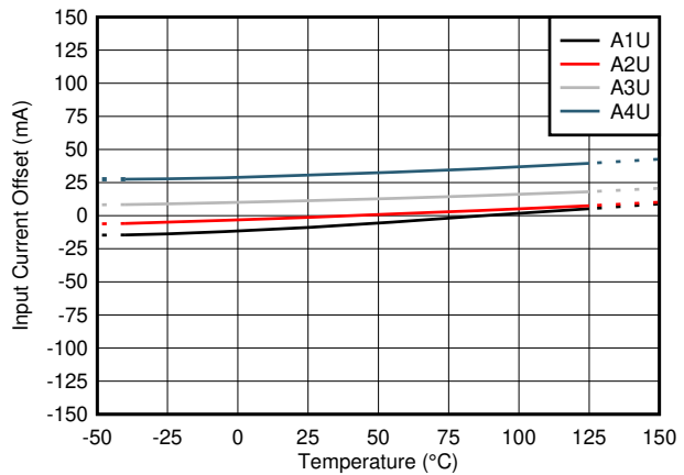
Figure 6-4. TMCS1101AxU-Q1 Input Offset Current vs Temperature
