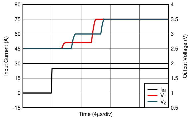
Figure 8-12. Transient Response to Input-Current Step Sufficient for 1V Output Swing
