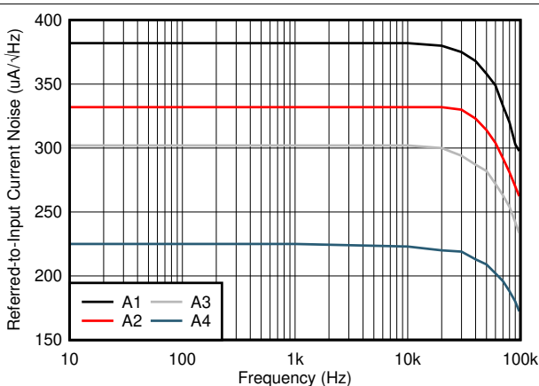
Figure 6-16. Input-Referred Noise vs Frequency
