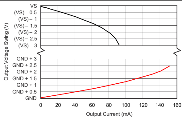
Figure 6-12. Output Swing vs Output Current
