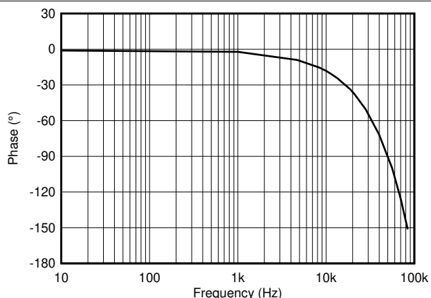
Figure 6-10. Phase vs Frequency, All Gains
