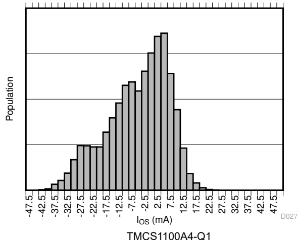
Figure 6-8. Input Offset Current Production Distribution
