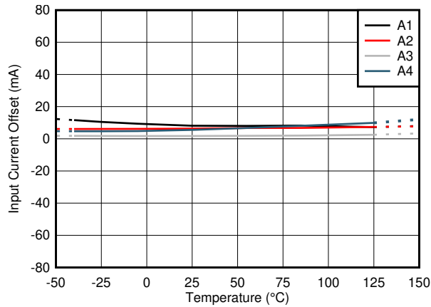
Figure 8-2. Offset Error Drift Across Temperature
