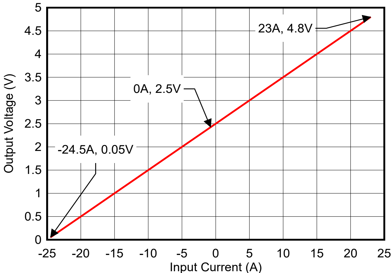
Figure 9-4. Application Example Design Transfer Curve
