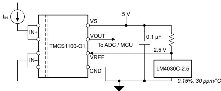
Figure 9-3. TMCS1100 Example Current-Sense System Design
