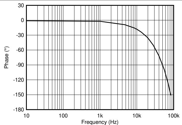
Figure 8-8. Normalized Phase, All Variants
