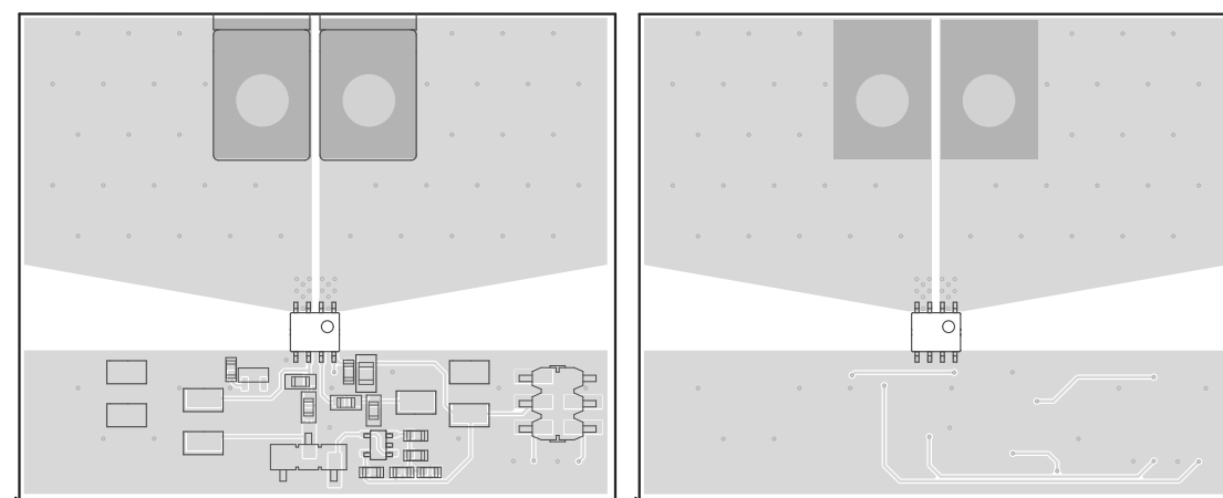
Figure 9-7. Recommended Board Top (Left) and Bottom (Right) Plane Layout
