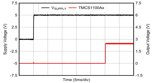
Figure 6-20. Startup Transient Response
