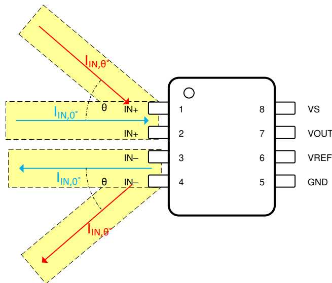
Figure 9-5. Magnetic Field Generated by Input Current Trace
