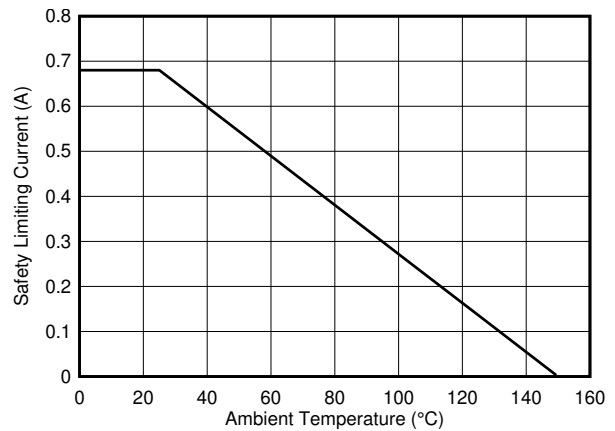
Figure 6-23. Thermal Derating Curve for Safety-Limiting Current, Side 2
