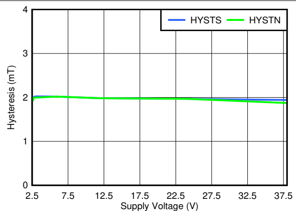
Figure 7-6. TMAG5123B Hysteresis vs Supply Voltage
