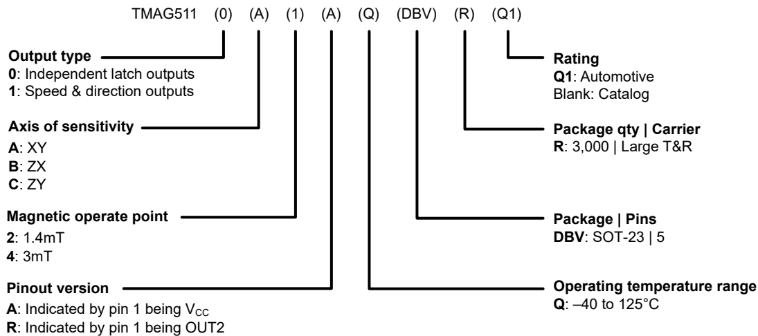
Figure 9-1. Device Nomenclature
