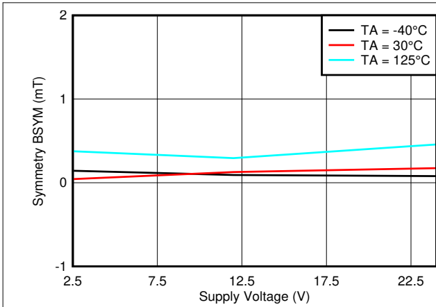
Figure 6-57. B_{SYM(Z)} vs V_{CC}
