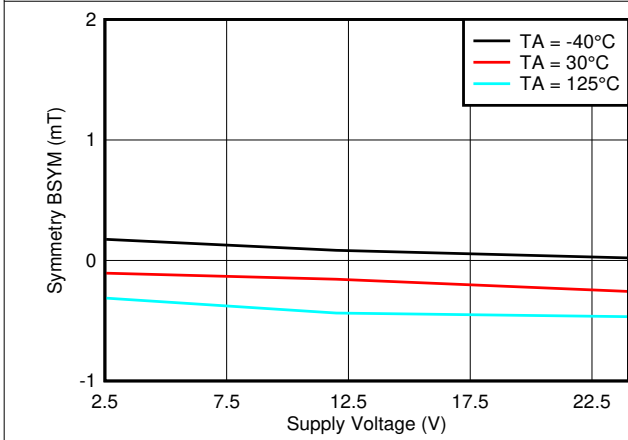
Figure 6-59. B_{SYM(X)} vs V_{CC}
