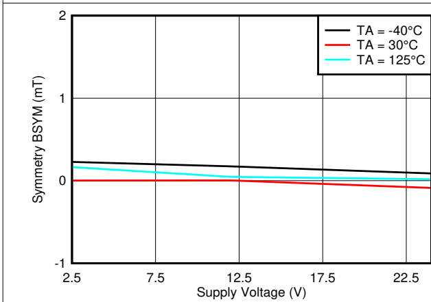
Figure 6-61. B_{SYM(Y)} vs V_{CC}
