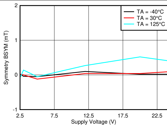
Figure 7-21. B_{SYM(X)} vs. V_{CC}
