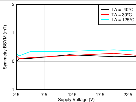
Figure 7-19. B_{SYM(Z)} vs. V_{CC}
