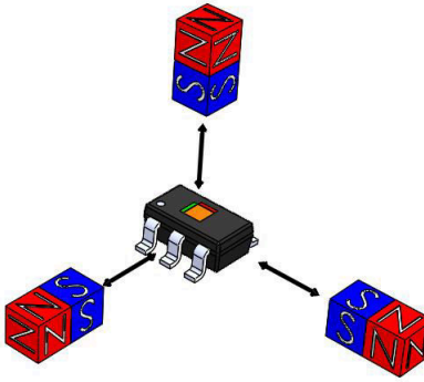
Figure 8-4. Axis Polarities
