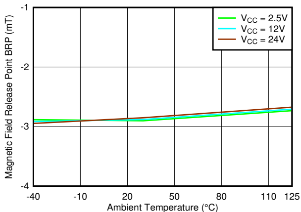
Figure 7-42. B RP_Z Threshold vs. Temperature
