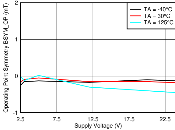
Figure 7-25. BSYM_OP(ZX) vs. V CC
