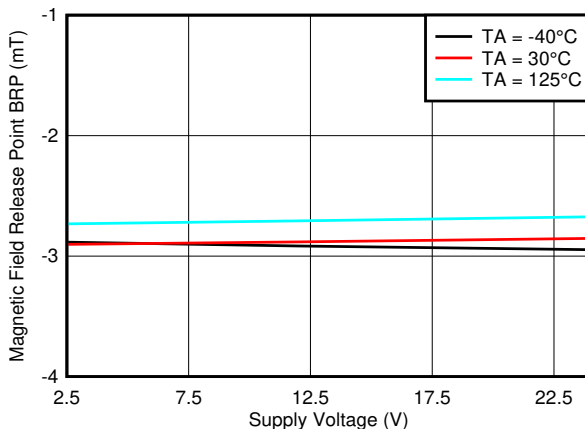
Figure 7-41. B RP_Z Threshold vs. V CC
