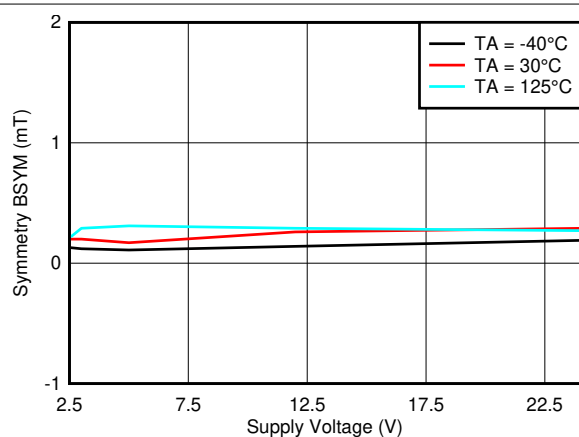
Figure 7-23. B_{SYM(Y)} vs. V_{CC}
