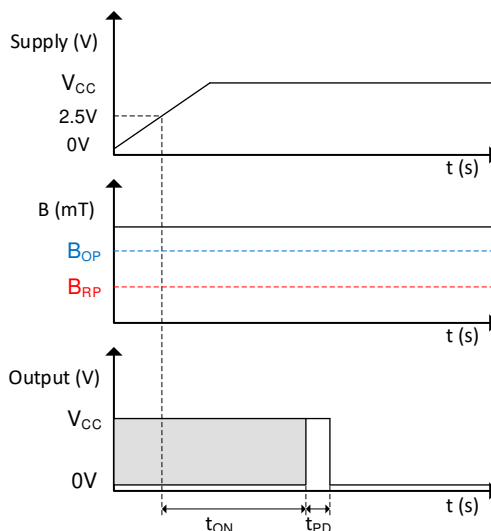
Figure 8-18. Power-On Time When B > B_{OP}
