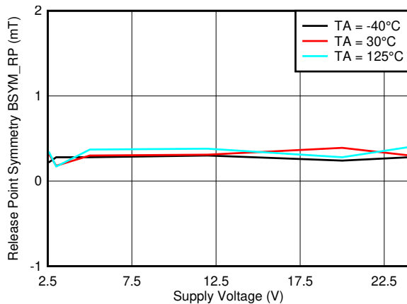
Figure 7-27. BSYM_RP(ZX) vs. V CC
