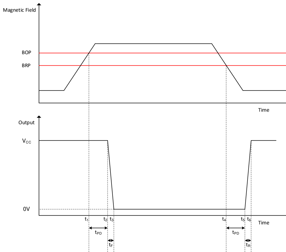
Figure 8-20. Propagation Delay
