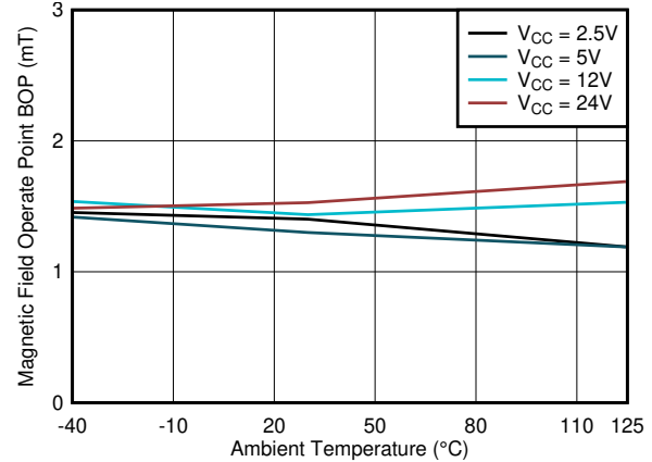
Figure 7-8. BOP_X Threshold vs. Temperature
