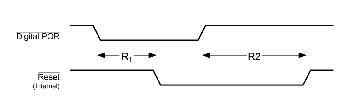
Figure 26-9. Digital Power-On Reset Timing
