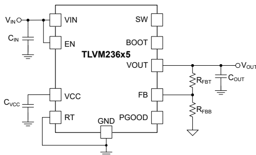
Typical Schematic
