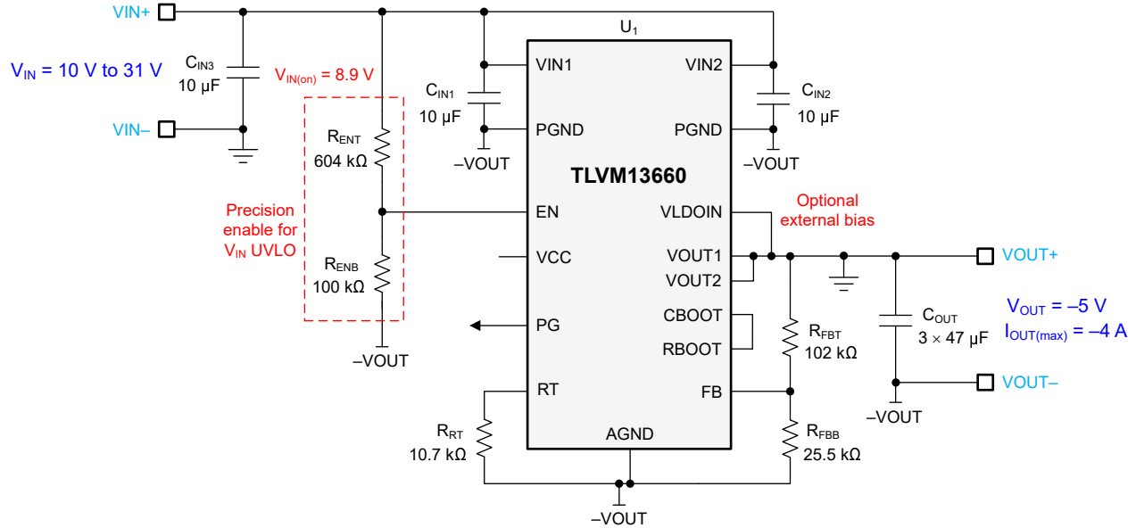
Figure 9-12. Circuit Schematic
