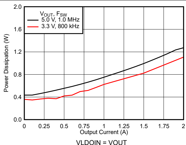
Figure 7-17. Power Dissipation
