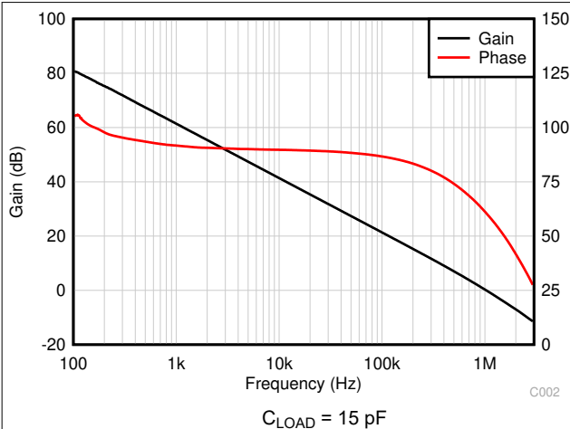
Figure 6-7. Open-Loop Gain and Phase vs Frequency
