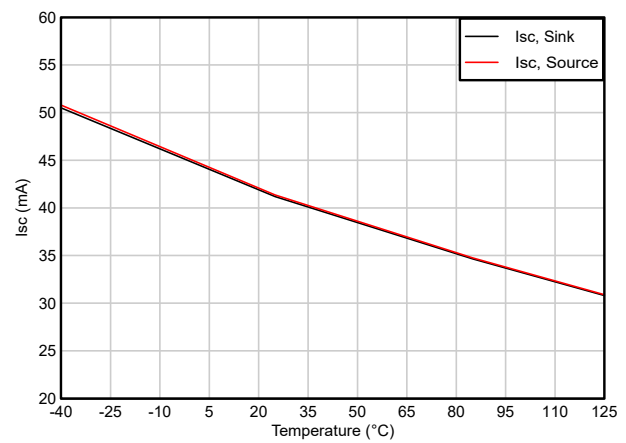
Figure 5-46. Short-Circuit Current vs Temperature
