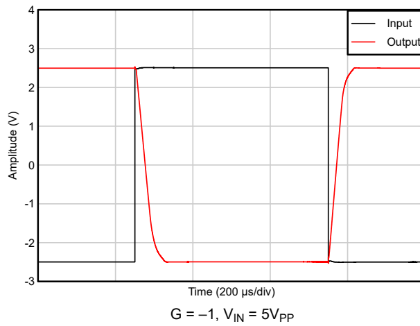
Figure 5-43. Large-Signal Step Response
