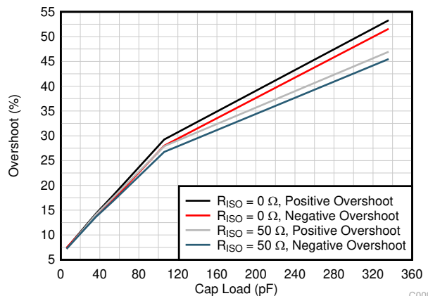
Figure 7-4. Small-Signal Overshoot vs Capacitive Load (100-mV Output Step, G = 1 )
