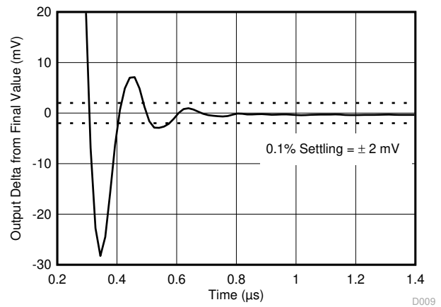
C_L = 100\text{pF} G = +1\text{V}/\text{V} Figure 6-28. Negative Large-Signal Settling Time
