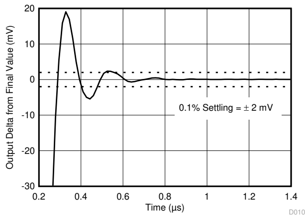
C_L = 100\text{pF} G = +1\text{V}/\text{V} Figure 6-27. Positive Large-Signal Settling Time
