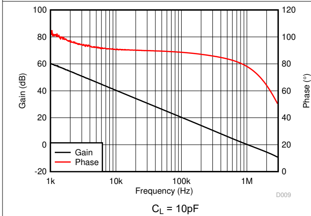
Figure 6-9. Open-Loop Gain and Phase vs Frequency
