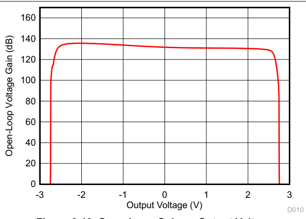
Figure 6-10. Open-Loop Gain vs Output Voltage
