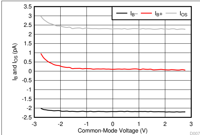
Figure 6-7. I_B and I_{OS} vs Common-Mode Voltage
