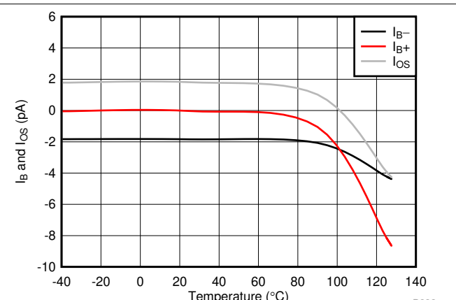
Figure 6-6. I_B and I_{OS} vs Temperature
