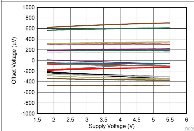
Figure 6-5. Offset Voltage vs Supply Voltage
