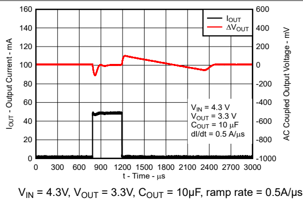
Figure 5-15. I_{OUT} Transient From 1mA to 50mA
