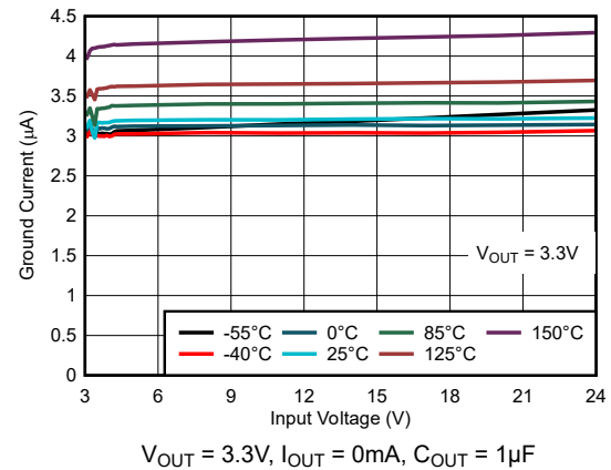
Figure 5-8. Ground Current vs V_{IN}
