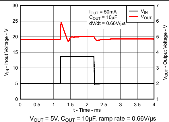
Figure 5-18. V_{IN} Line Transient (5V to 14V for V_{OUT} = 5\text{V} )
