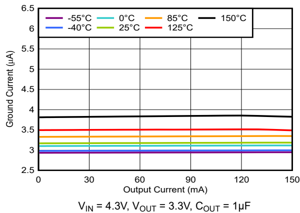
Figure 5-9. Ground Current vs I_{OUT}
