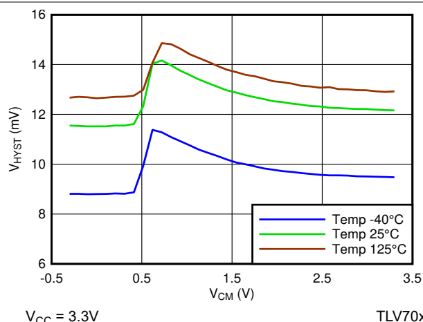
Figure 5-15. Hysteresis vs V_{CM}
