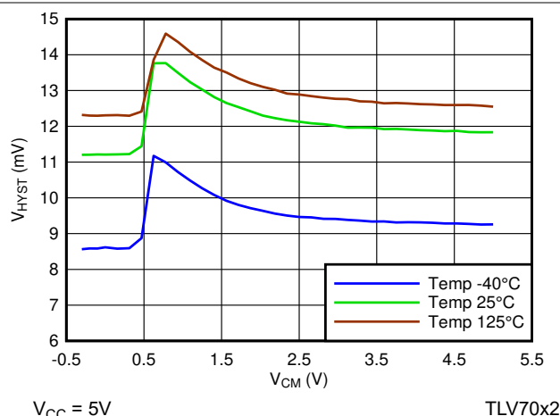
Figure 5-16. Hysteresis vs V_{CM}
