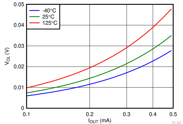
Figure 16. Output Voltage Low vs. Output Sink Current
