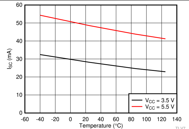
Figure 18. Output Short-Circuit (Sink) Current vs. Temperature
