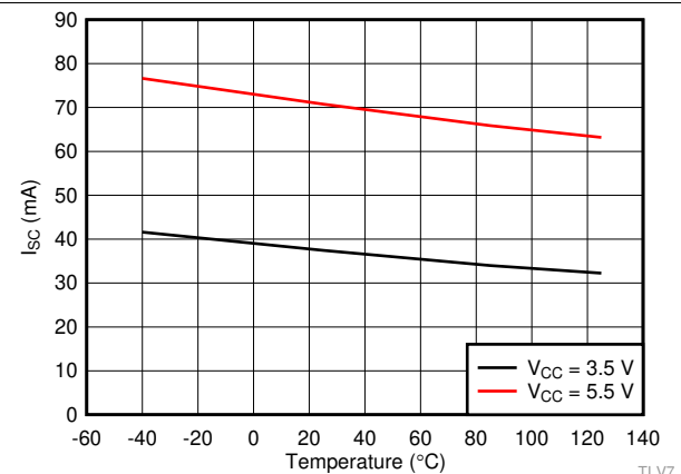
Figure 19. TLV701x Output Short-Circuit (Source) Current vs. Temperature
