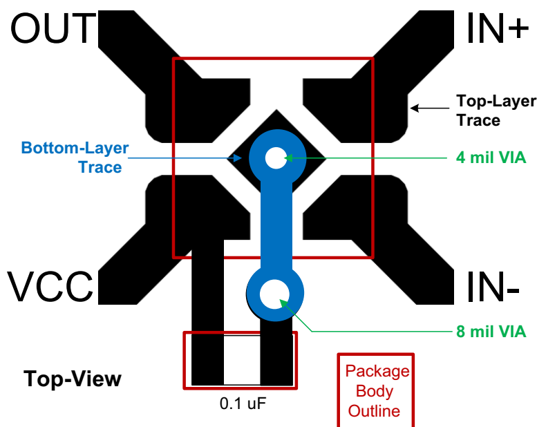
Figure 42. Layout Example
