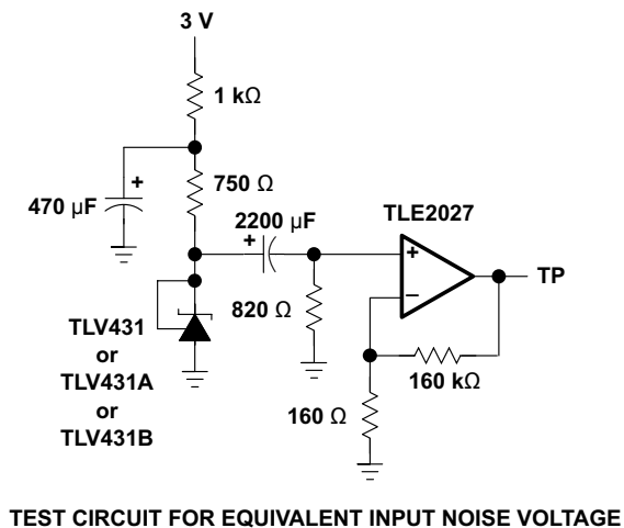
Figure 5-12. Equivalent Input Noise Voltage
