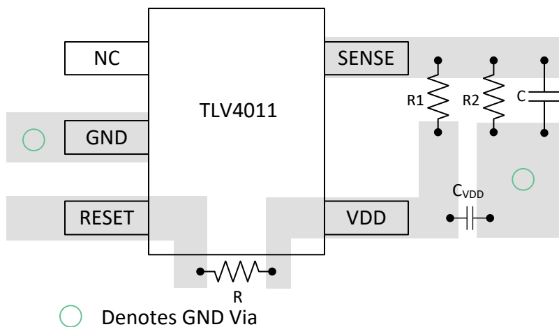
Figure 10-1. Layout Example
