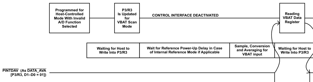
Figure 73. Host-Controlled VBAT Scan Mode
