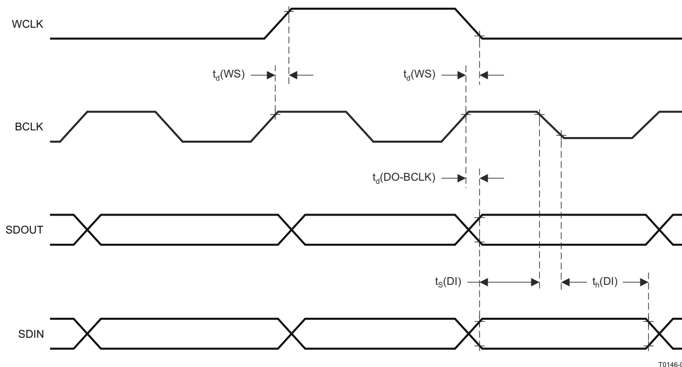
Figure 6-3. DSP Timing in Master Mode
