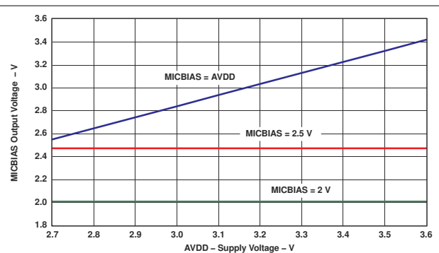
Figure 11-3. MICBIAS Output Voltage vs AVDD
