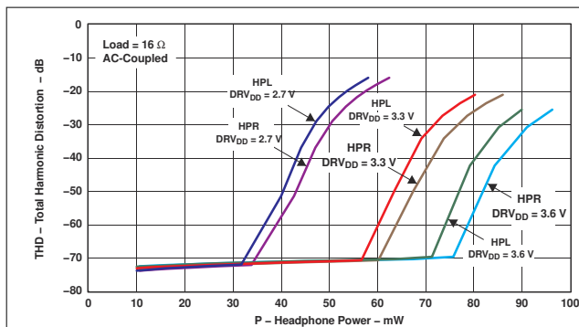
Figure 11-2. THD vs Headphone Power, 16- \Omega Load
