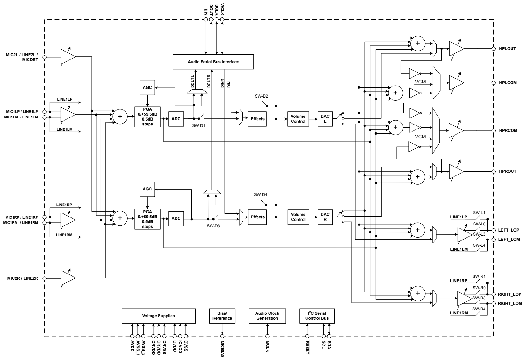
Figure 10-1. Functional Block Diagram
