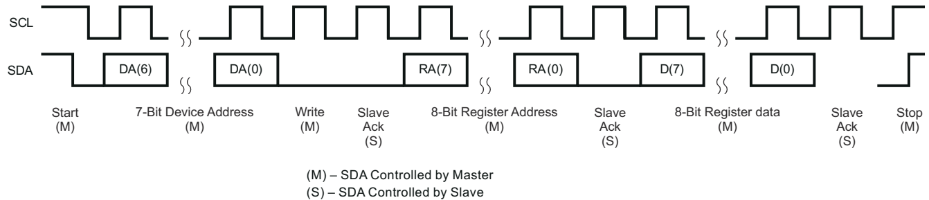
Figure 10-24. I²C Write
