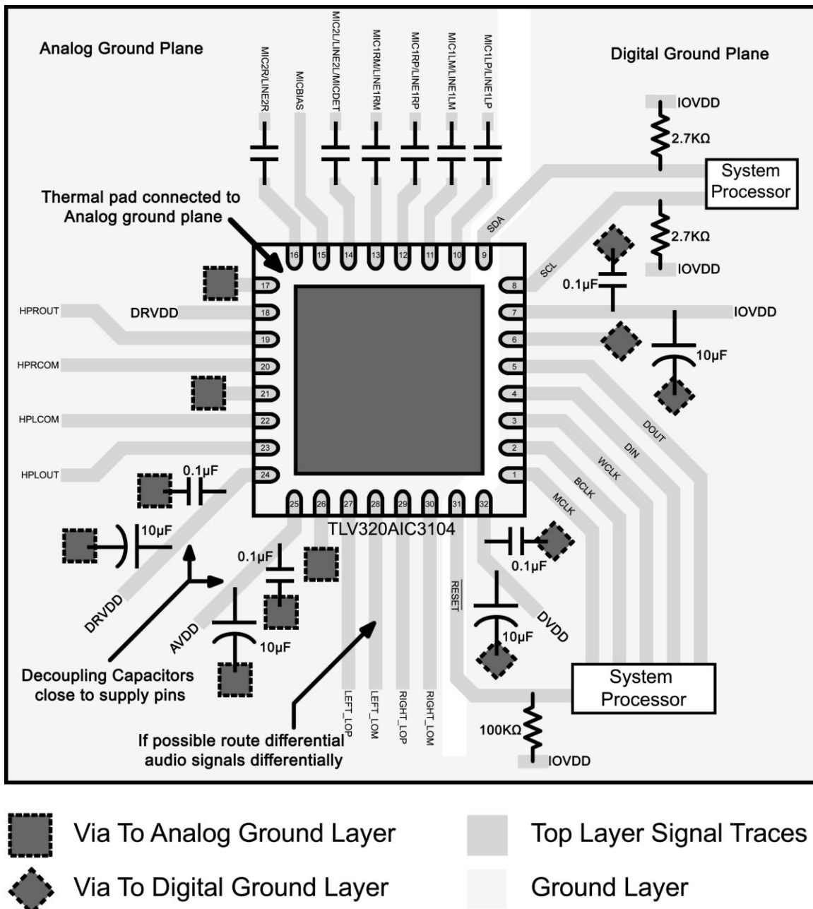
Figure 13-1. Layout Example
