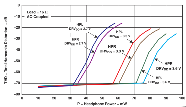
Figure 8-5. THD vs Headphone Power, 16-Ω Load
