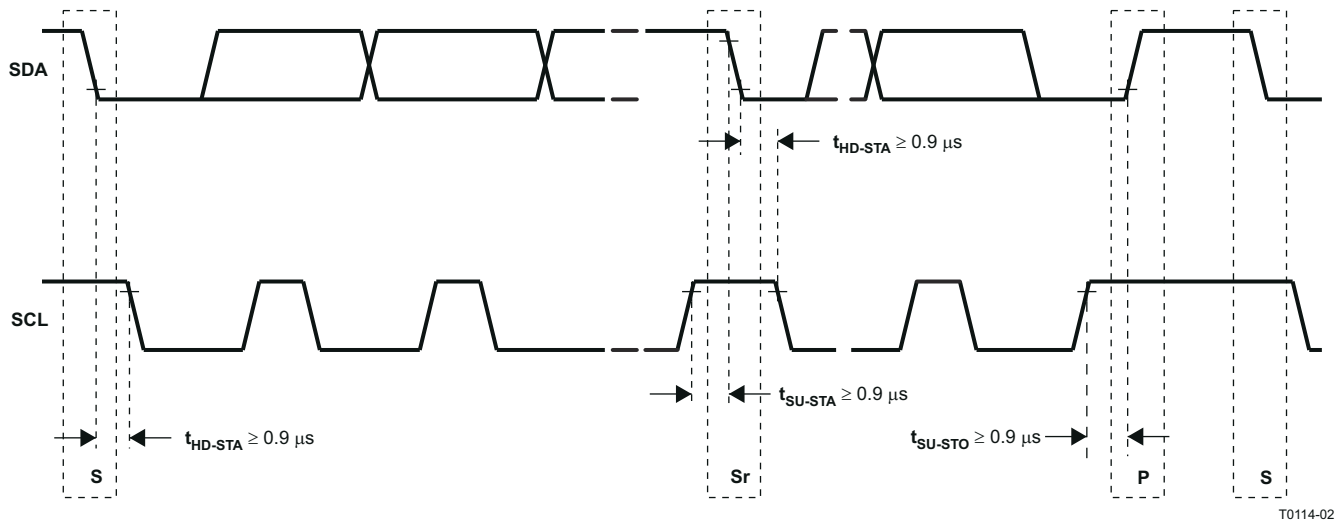
Figure 10-23. I 2 C Interface Timing
