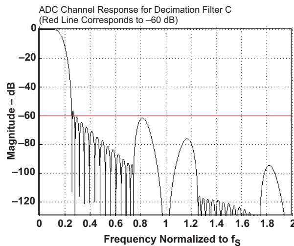
Figure 7-14. ADC Decimation-Filter-C Frequency Response
