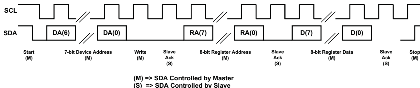
Figure 12. I²C Write
