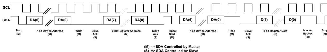
Figure 13. I²C Read
