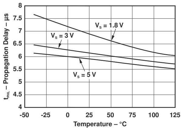
Figure 6-9. PROPAGATION DELAY ( t_{pHL} ) vs TEMPERATURE
