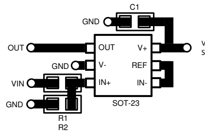
Figure 10-7. Layout Example
