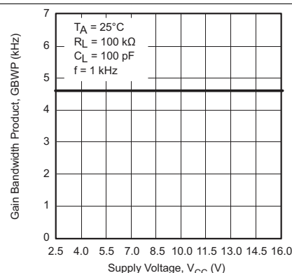
Figure 22. Gain Bandwidth Product vs Supply Voltage
