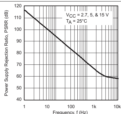
Figure 20. Power Supply Rejection Ratio vs Frequency
