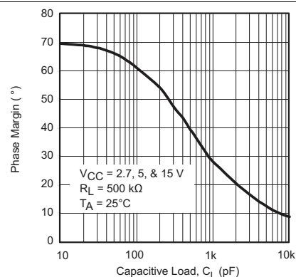
Figure 24. Phase Margin vs Capacitive Load
