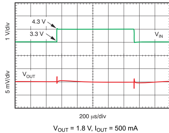
Figure 6-22. Line Transient Response
