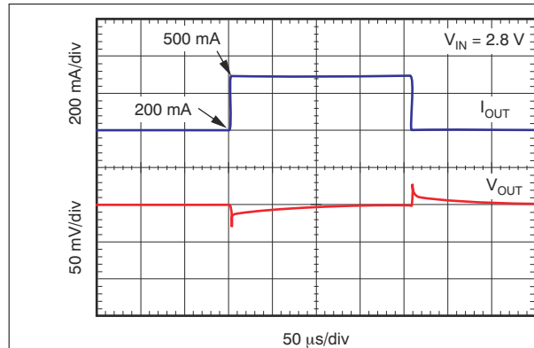
Figure 8-2. Load Transient Response 200 mA to 500 mA, C_{OUT} = 1\ \mu\text{F}
