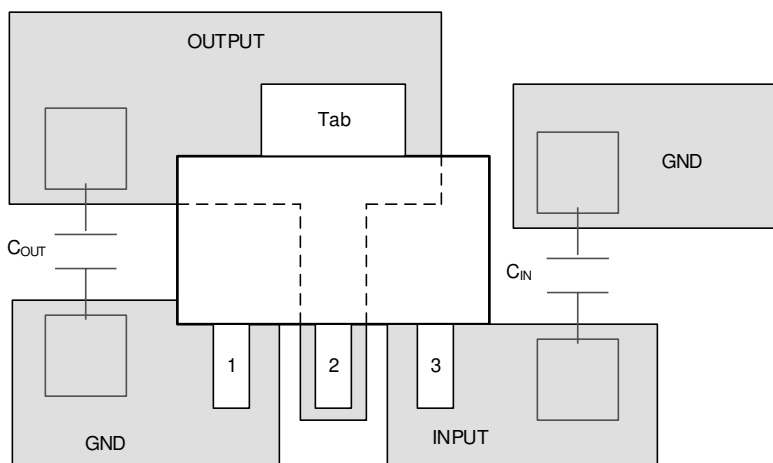
Figure 8-4. Layout Example
