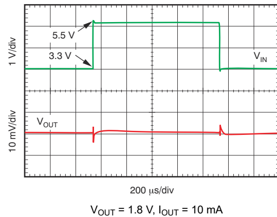
Figure 6-24. Line Transient Response
