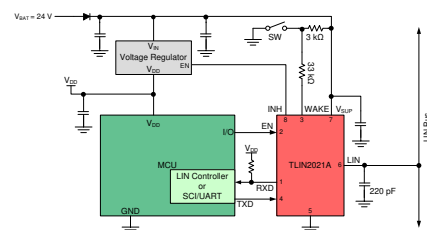
Simplified Responder Node Schematic
