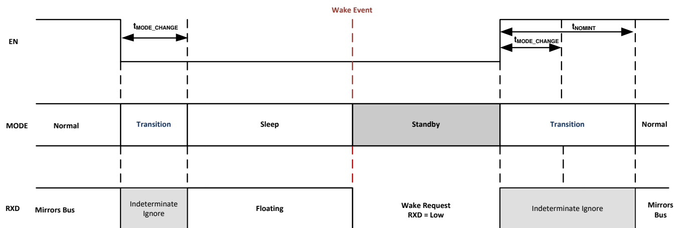
Figure 8-14. Mode Transitions
