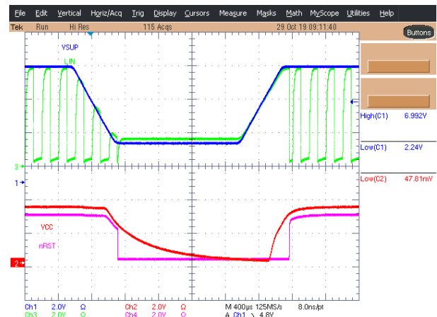
Figure 10-17. TLIN10283-Q1 Brownout
